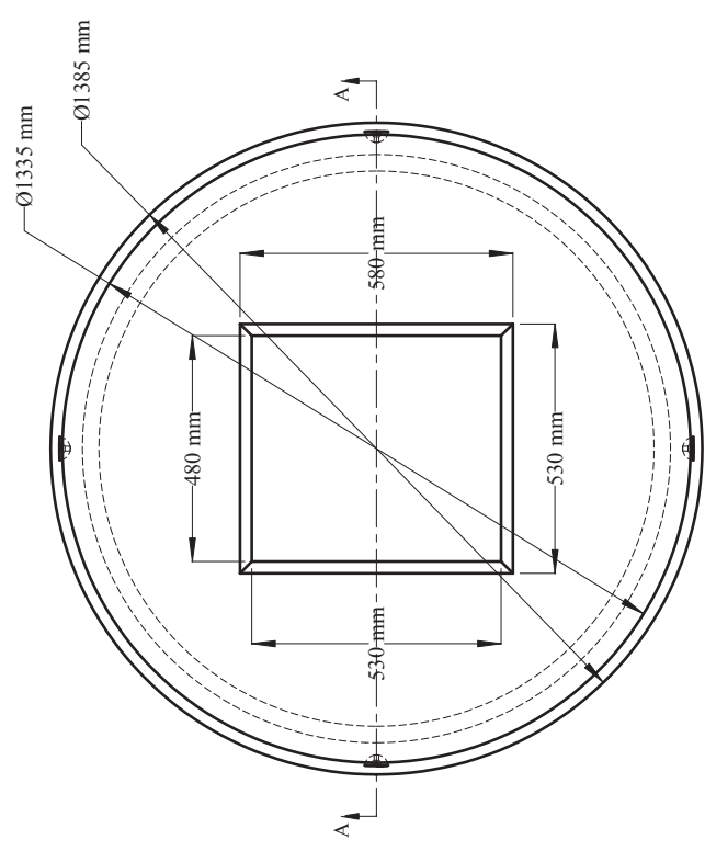
PLAN VIEW
